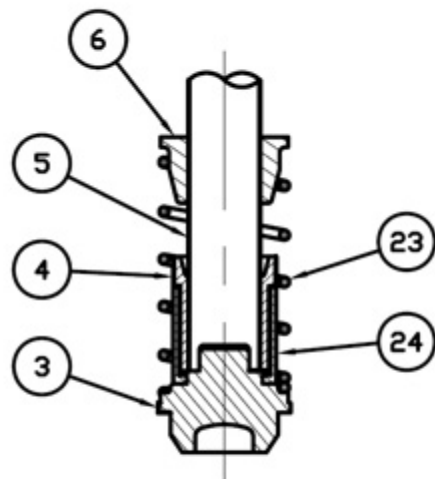
ENLARGED VIEW OF STOP CHECK INTERNALS
