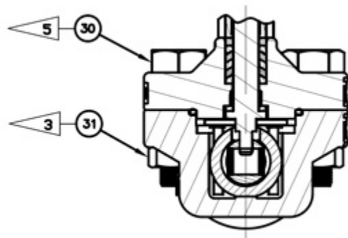
PARTIAL SECTION A - A
